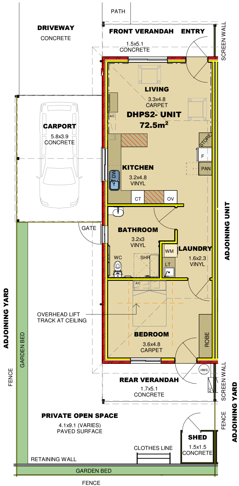
DHPS2- HIGH PHYSICAL SUPPORT UNIT SCALE 1:100 @ A4
